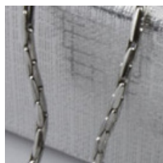
Block Chain
